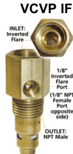
VCVP IF Inlet: Inverted Flare Fitting Outlet: Female NPT Port: 1/8" NPT & 1/8" Inverted Flare Port
